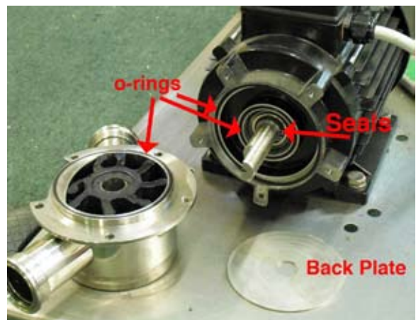
Fig. 4. Remove, clean, and lubricate pumphead regularly.
