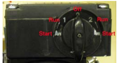
Fig. 1. Euro 30 5-position switch. Far right (or left) is START.
