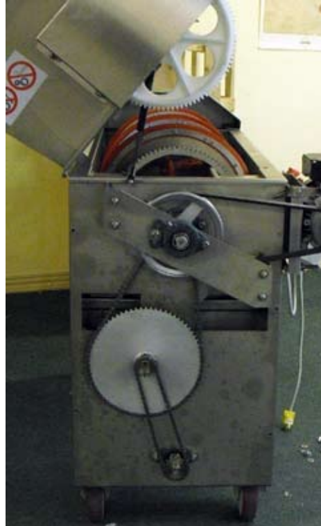
Fig. 8. Remove end cover annually and lubricate chains and gears. Do not grease the V-belts. Do not wash down these components.
