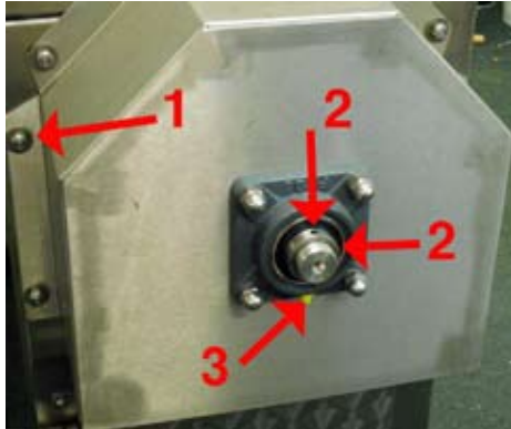
Fig. 3. Remove the destemming shaft and basket. Remove the nuts (indicated by the “1”). Loosen the set screws (indicated by the “2”s). Now the cover can be removed. The destemming shaft is simply twisted and pulled out. The destemming basket is then lifted out. All internal components are now easily accessible.
