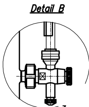
3-way valve Letina NW15 with holender DN15 (DIN11851)
