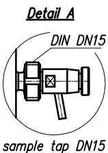
sample tap DN15
